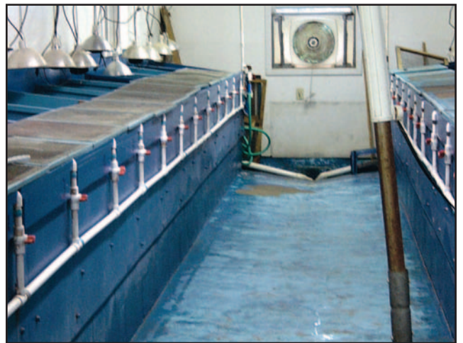
Fig 36.42 | Brooder room.
